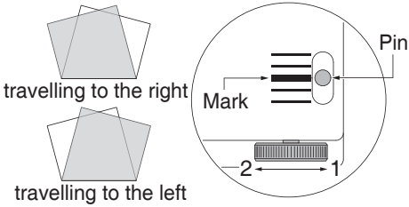
Paper feed table adjustment knob
